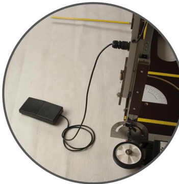
The foot operated switch is attached to the cutting bow.
